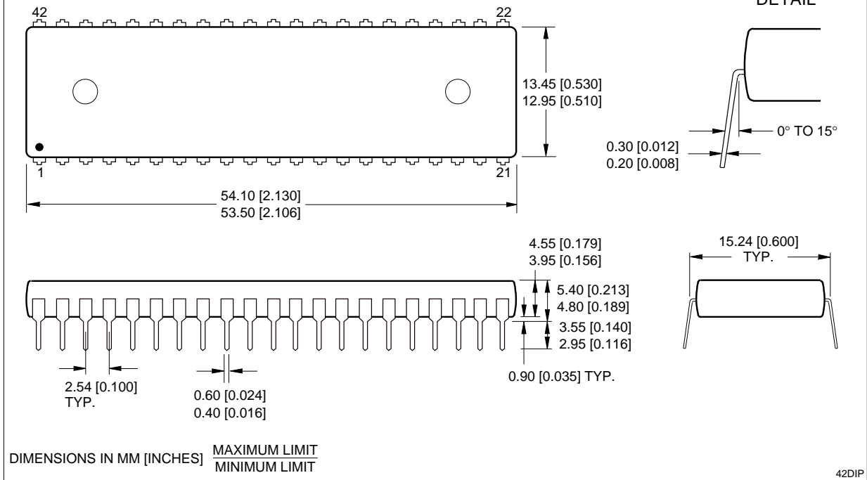
42-pin, 600-mil DIP
