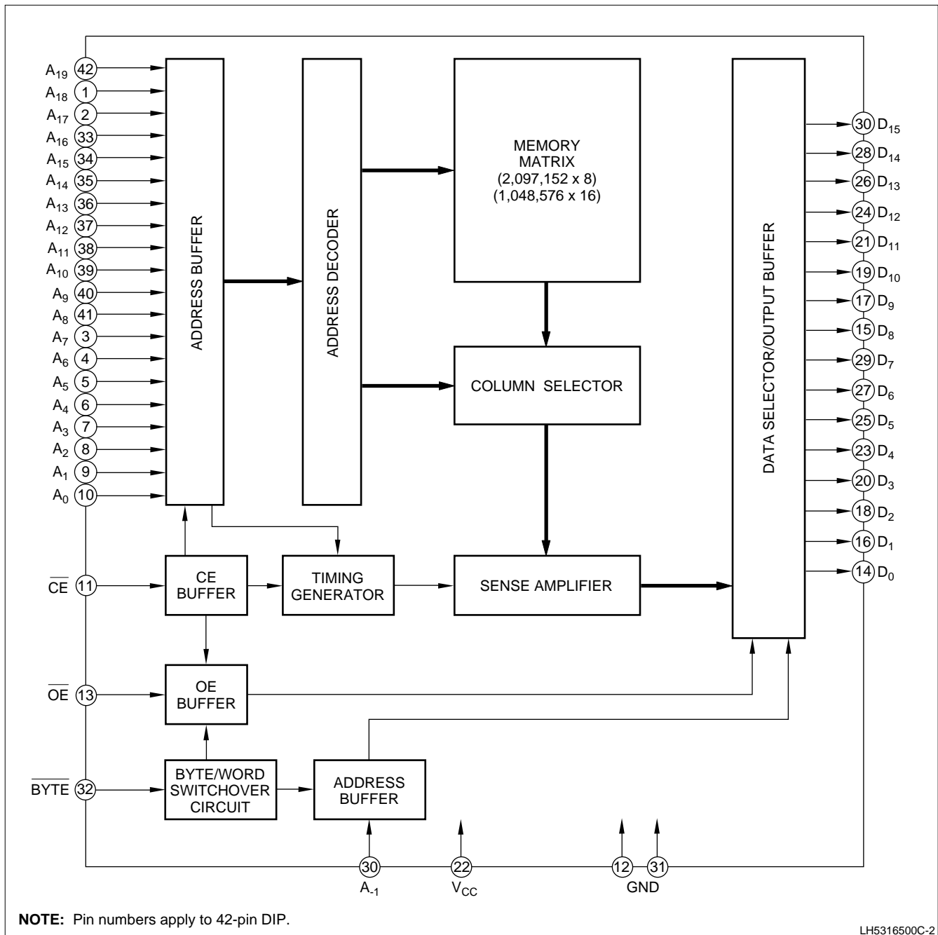
Figure 3. LH5316500C Block Diagram
